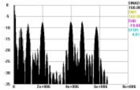
Figure 9. This FFT of the multiburst signal shows frequency on the horizontal axis, allowing a measurement of the bandwidth required for the burst of each frequency. This spectrum of the whole video signal indicates the bandwidth required to pass this signal without distortion.
